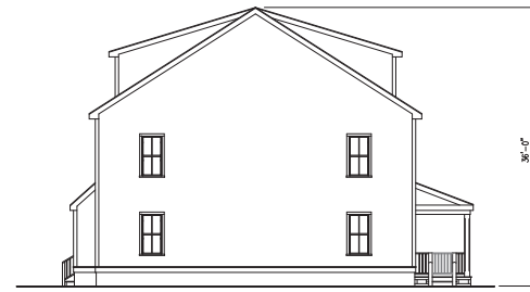
3 BUILDING B-6 - SIDE ELEVATION SCALE: 1/8" = 1'-0"
