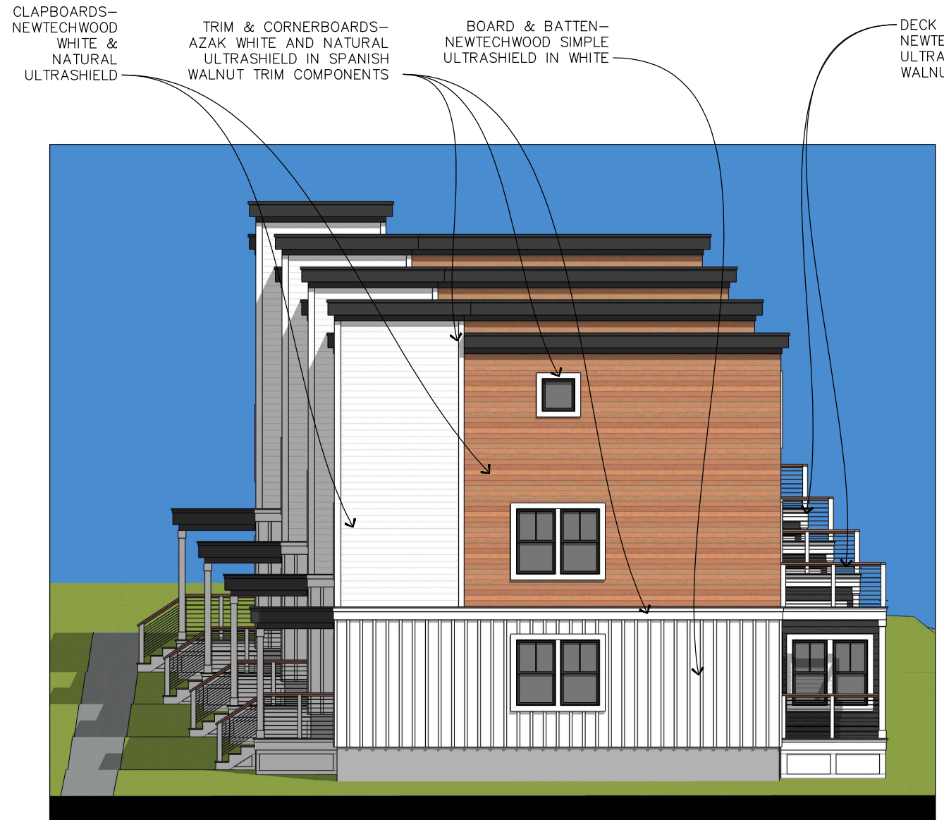
1 WEST ELEVATION SCALE: 3/32" = 1'-0"
