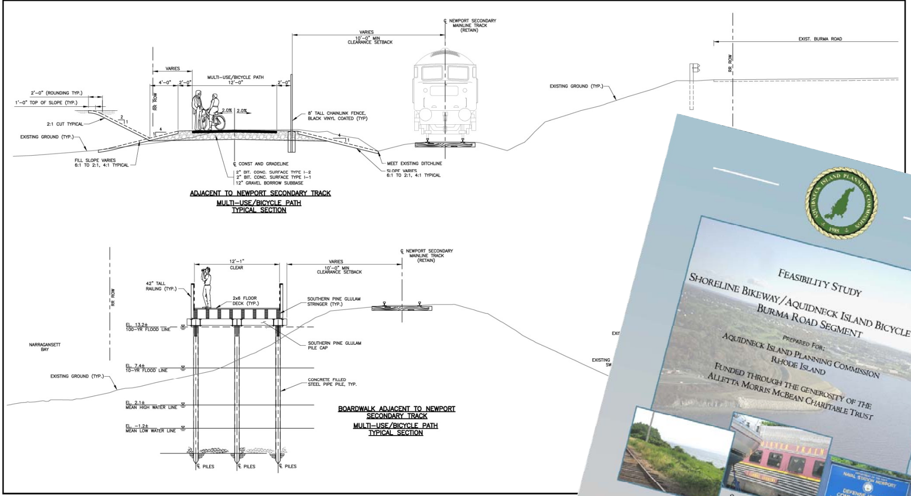
Figure No. 2 TYPICAL SECTIONS BURMA ROAD SEGMENT
