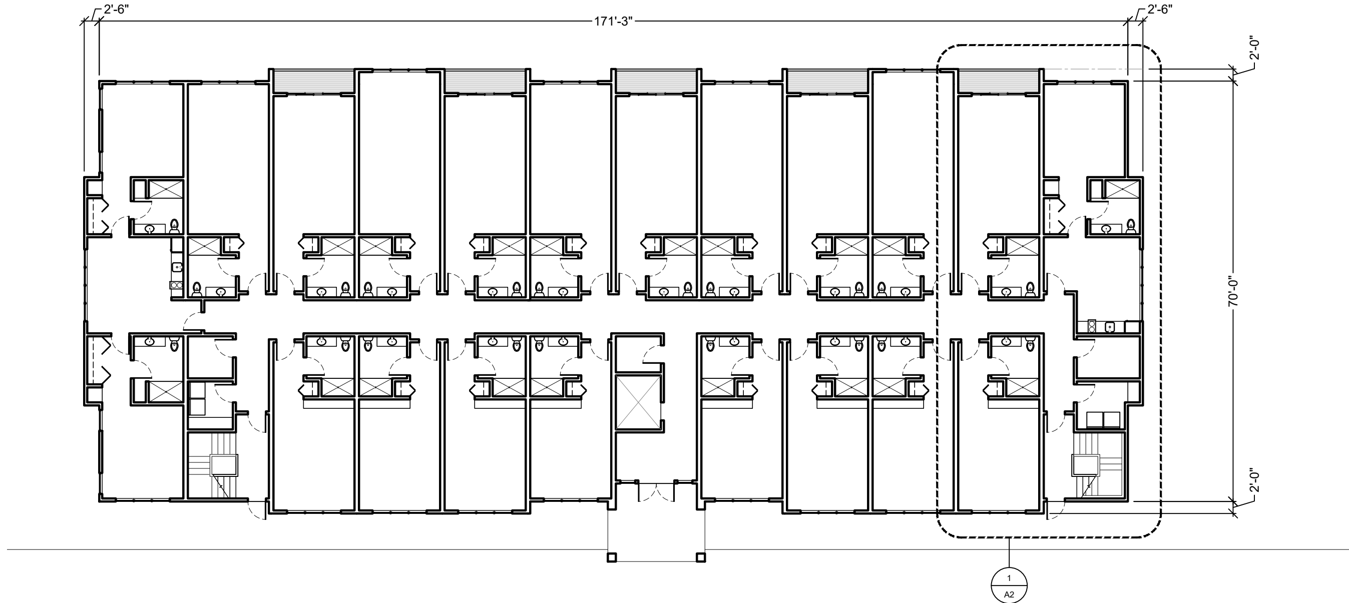
1 FIRST FLOOR PLAN A1 SCALE: 1/16" = 1'-0"
